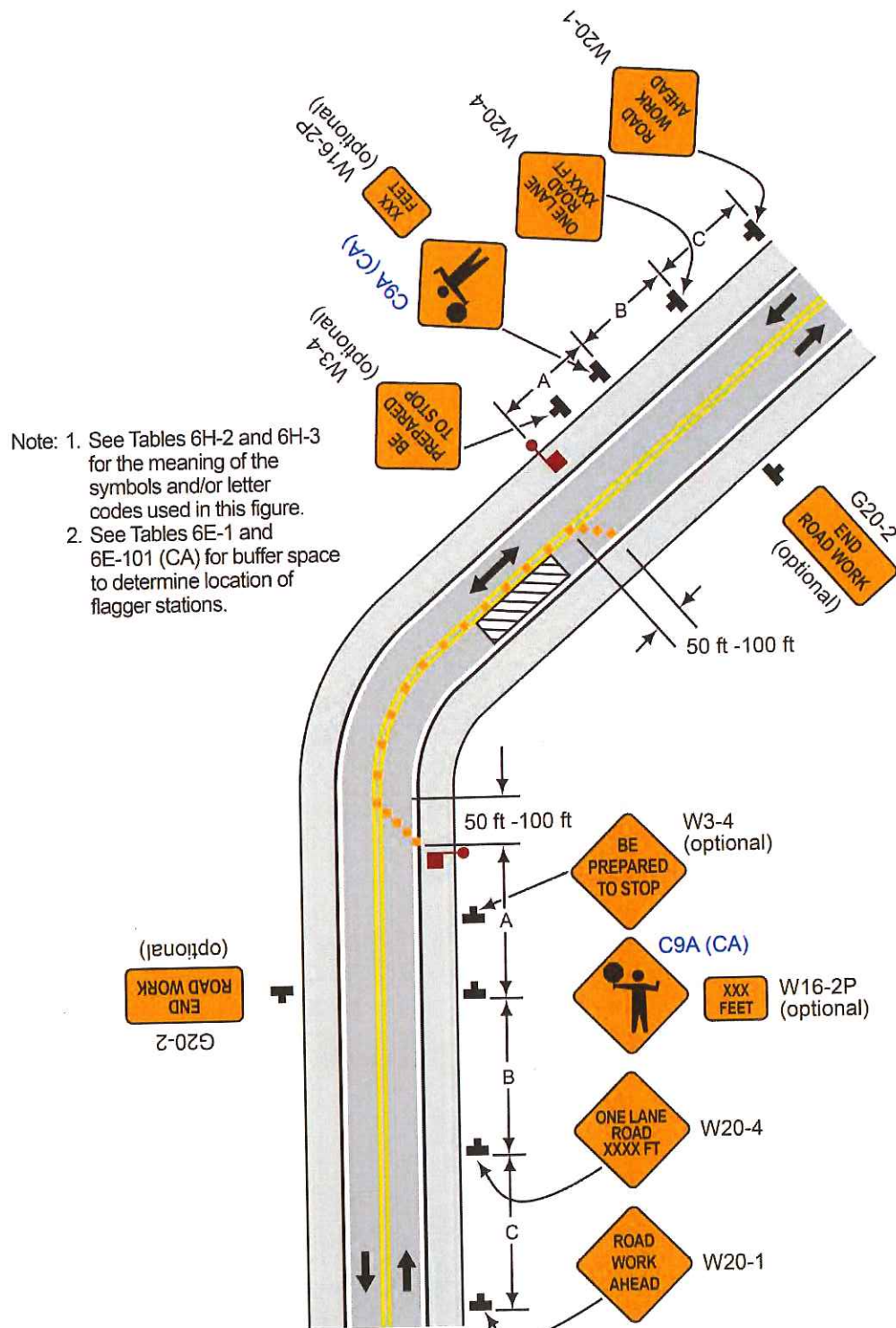
Typical Application 10
